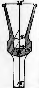
SECTION OF RIM OF 6 FT. WHEEL
